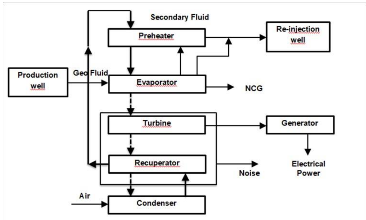
Figure 2-2. Process Flow Chart
