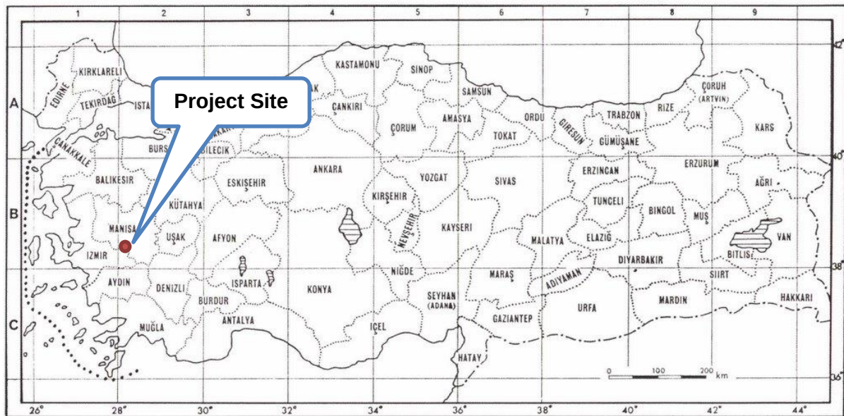
Figure 5-5. Grid System for Flora of Turkey
